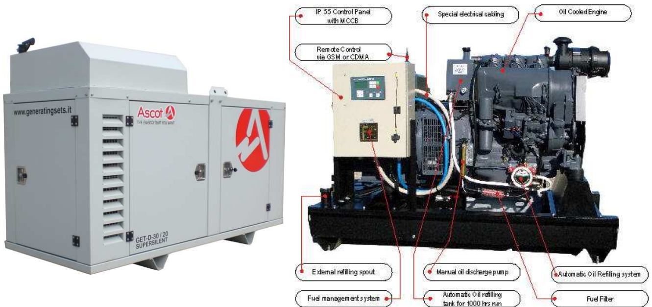
Diesel Generating sets 30-40 KVA Air cooled for Mobily project Saudi Arabia
